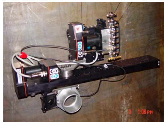
5085 scanner in a snowplow orientation
