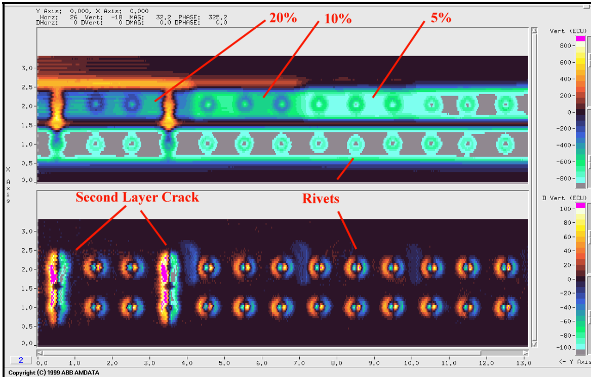
Eddy Current Image of simulated corrosion obtained AMDATA IntraSpect Eddy Current Imaging System
